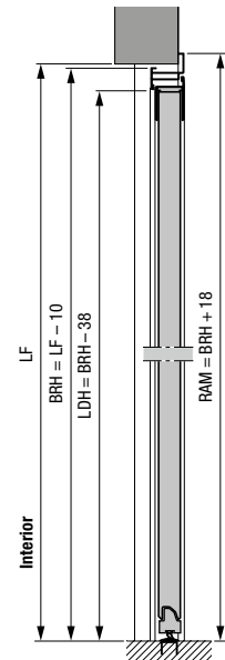
Side door with aluminium corner frame, profile type 2 External fitting
