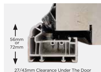
Two sizes of PVCu threshold.
